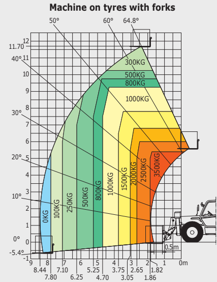
Rough terrain load chart standard EN1459 B
